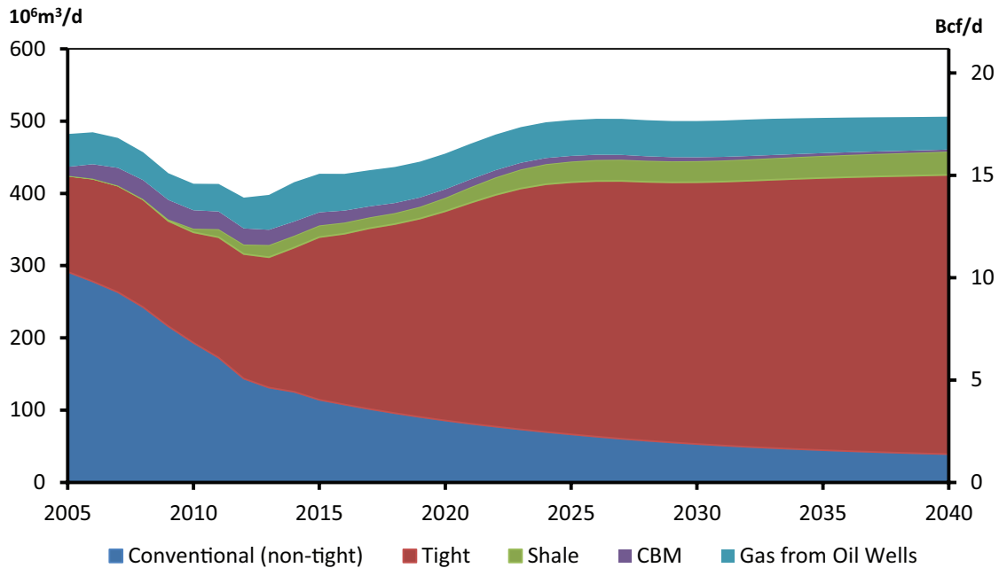
Natural Gas Production by Type, Reference Case
